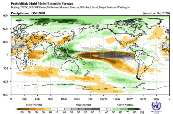
Figure 1. Probabilistic forecasts of surface air temperature and precipitation for the season October-December 2020. The tercile category with the highest forecast probability is indicated by shaded areas. The most likely category for below-normal, above-normal and near-normal is depicted in blue, red and grey shadings respectively for temperature, and orange, green and grey shadings respectively for precipitation. White areas indicate equal chances for all categories in both cases. The baseline period is 1993-2009.
